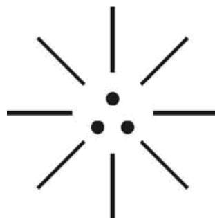
(Trisomy human)
