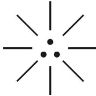
(GODLY PARTICLE)
